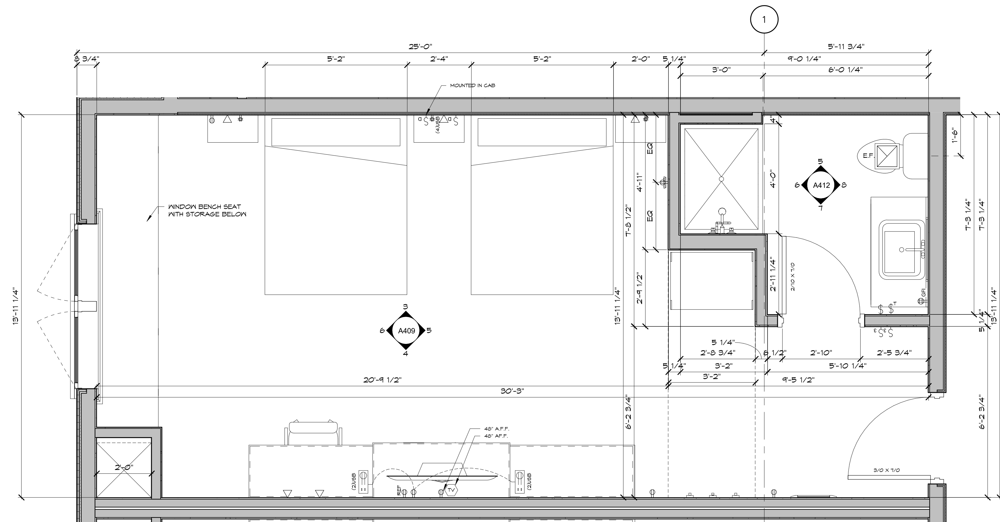
FLOOR PLAN - FIRST FLOOR - NEW - Callout 1 - Callout 2 1/2" = 1'-0"
