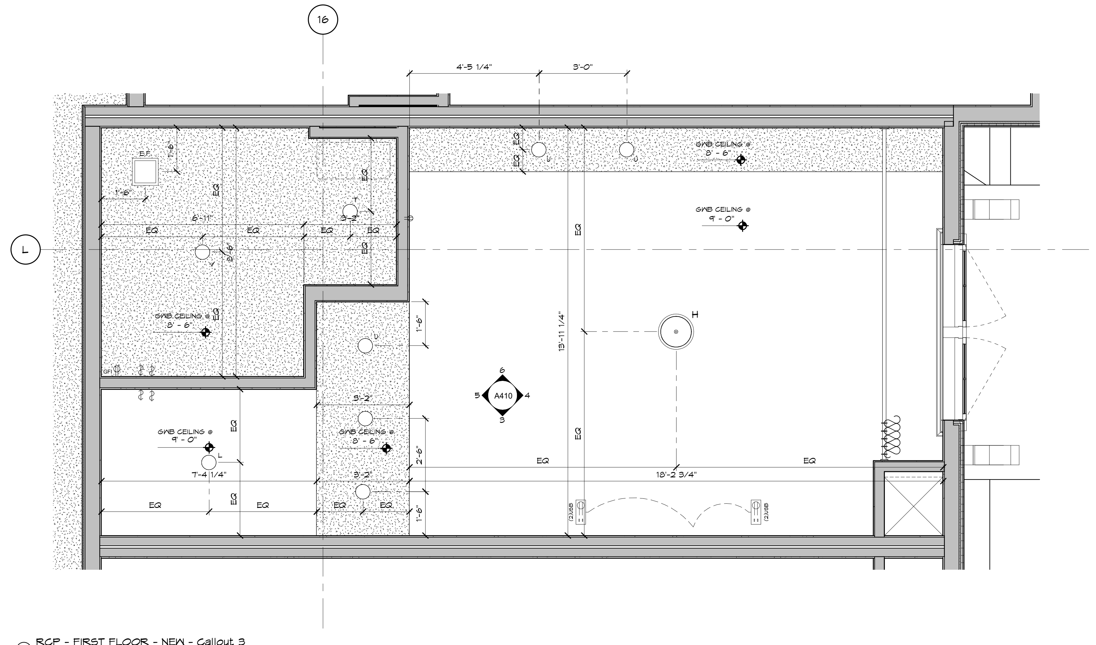
2 RCP - FIRST FLOOR - NEW - Callout 3 1/2" = 1'-0"
