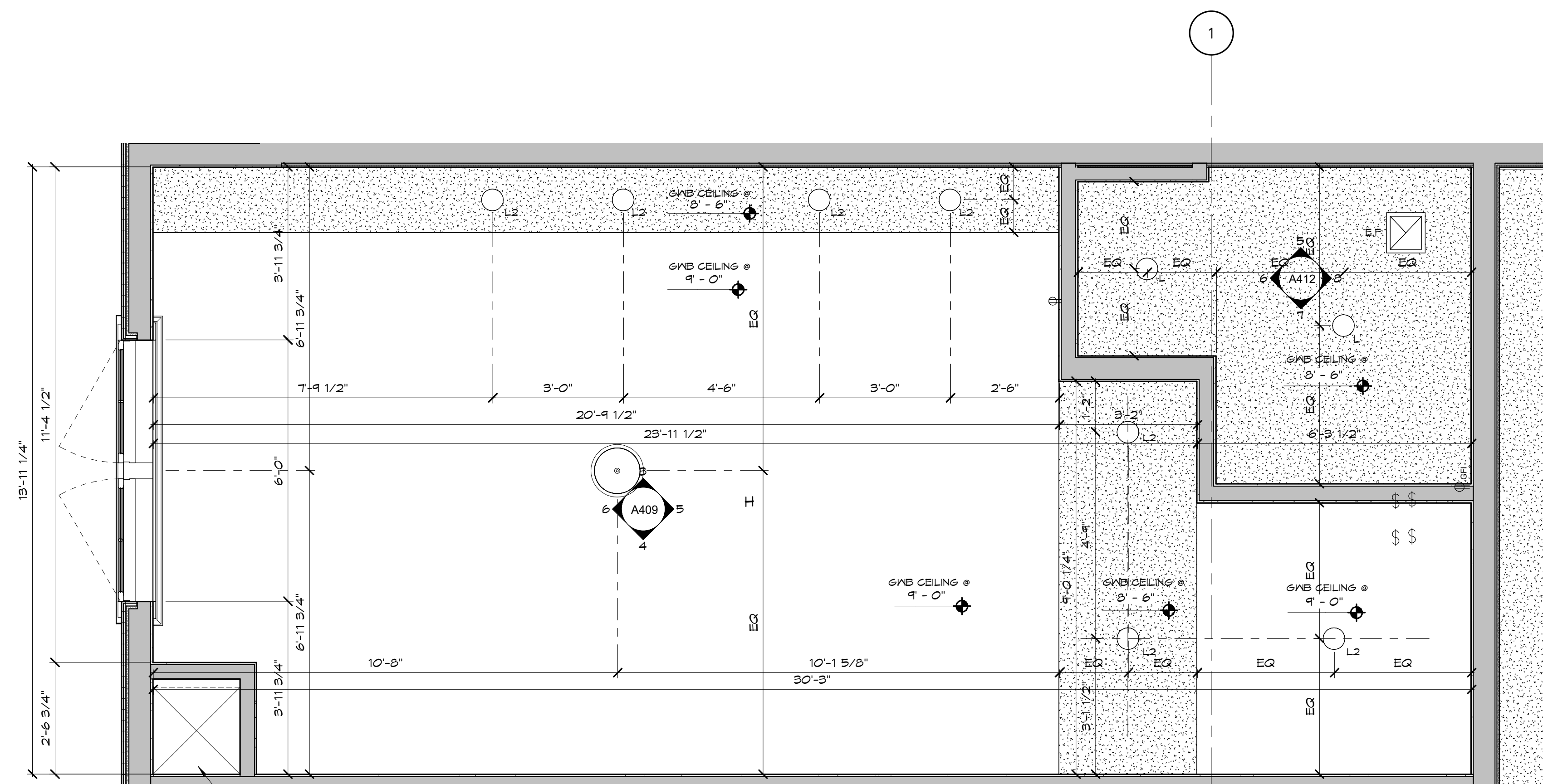
RCP - FIRST FLOOR - NEW - Callout 1 - Callout 2 1/2" = 1'-0"
