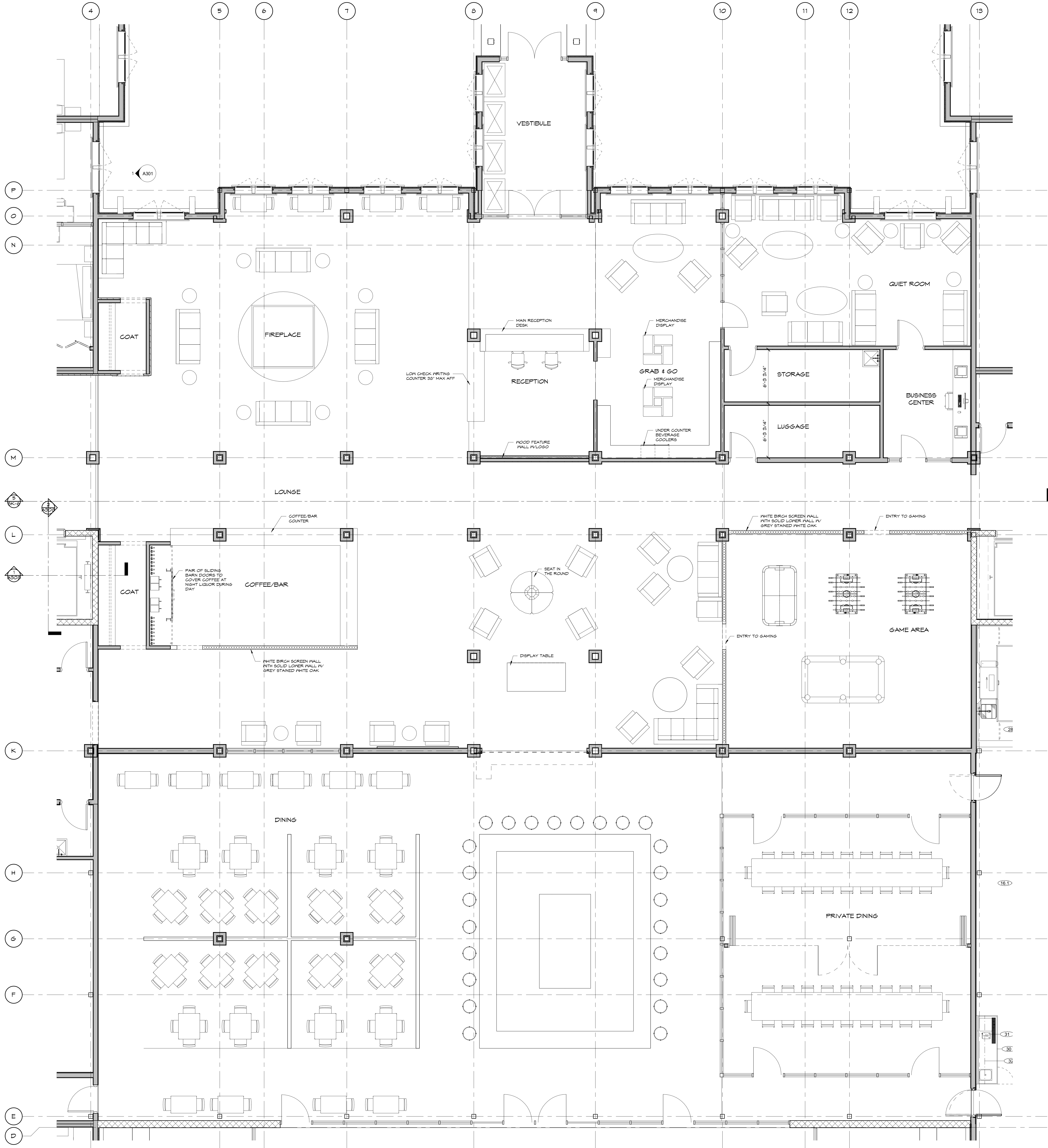
1 FLOOR PLAN - FIRST FLOOR - NEW - Callout 10 1/4" = 1'-0"
