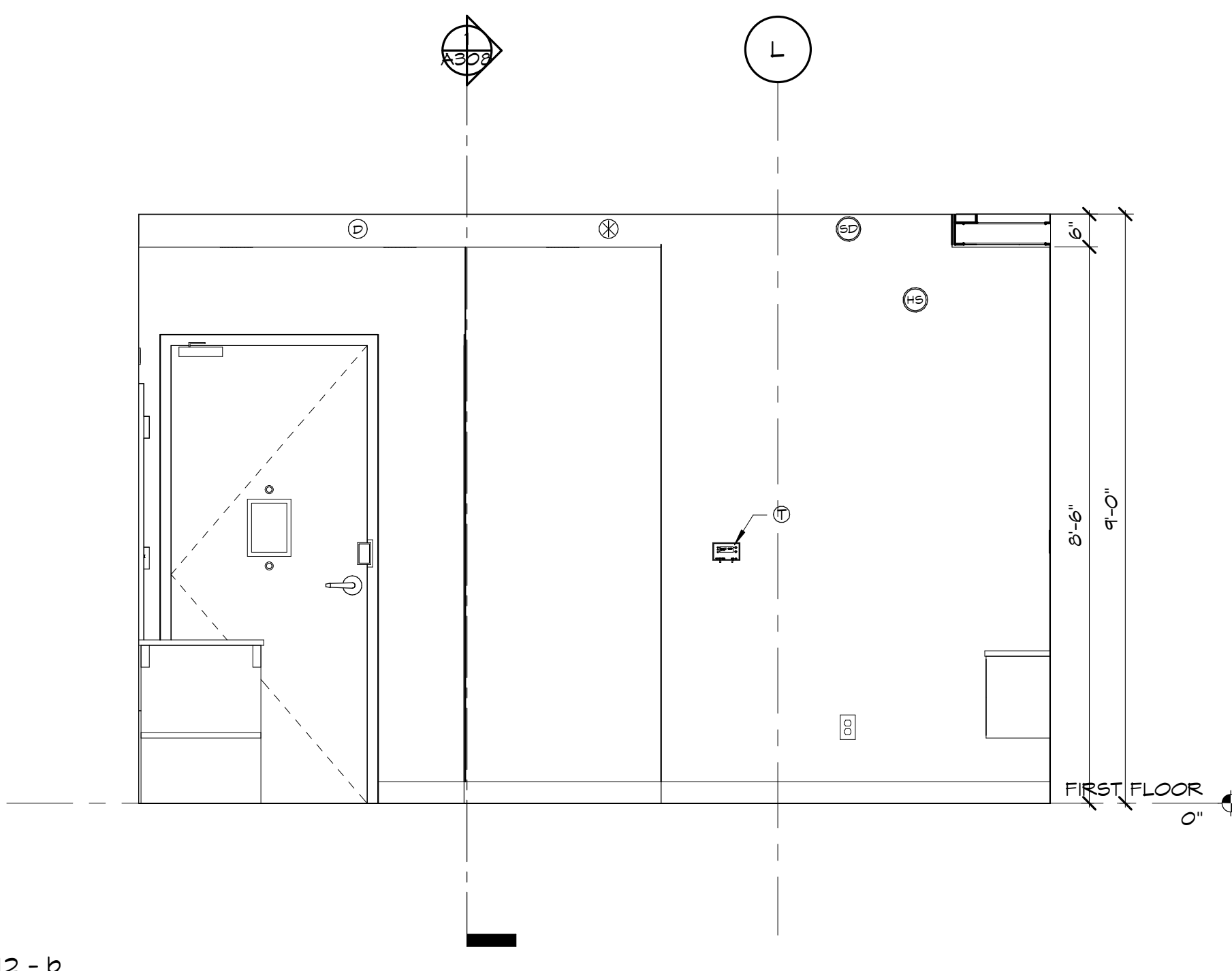
12 - b 1/2" = 1'-0"
