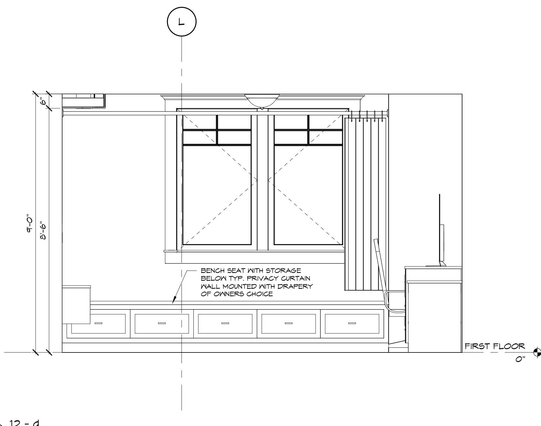
12 - d 1/2" = 1'-0"
