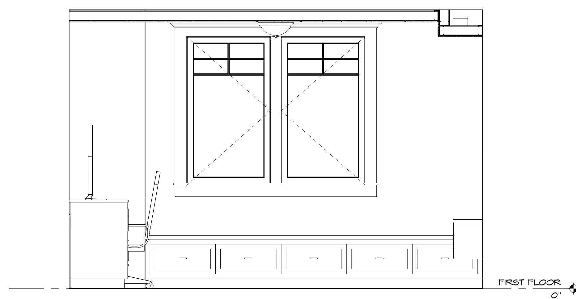
11 - b 1/2" = 1'-0"
